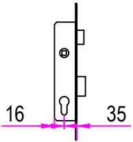
AKS14 DİLLİ KİLİT MOURTISE LOCK WITH CYLINDER
