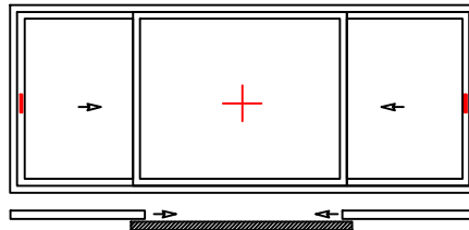
2 HAREKETLİ 1 SABİT KANAT 2 SLIDING 1 FIX SASH
